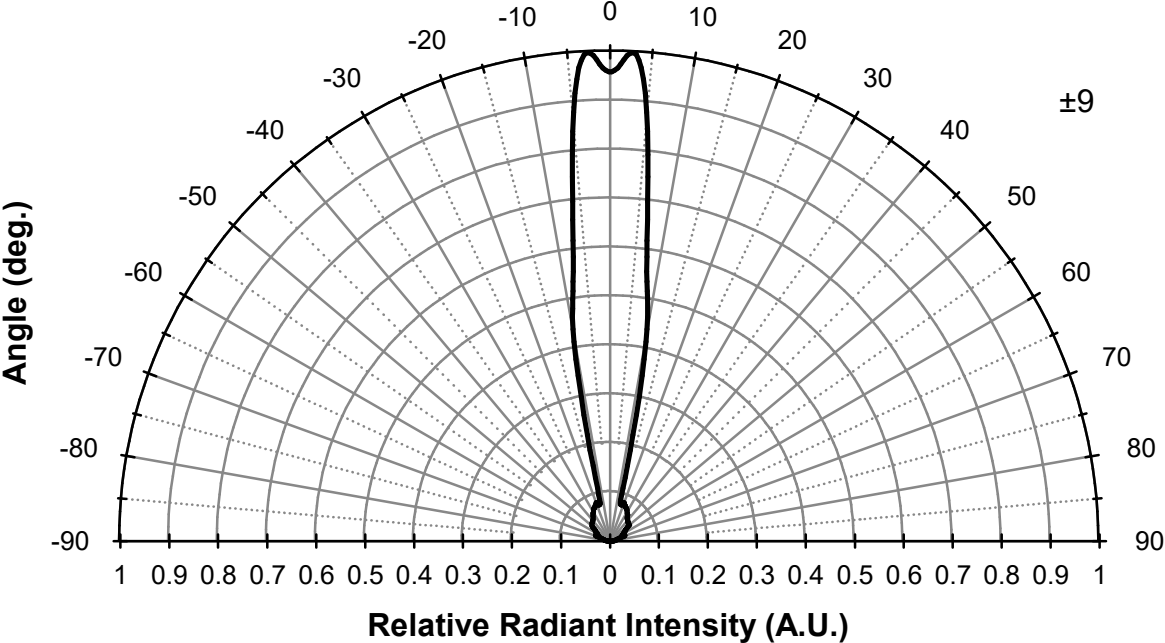
Radiation Characteristics
